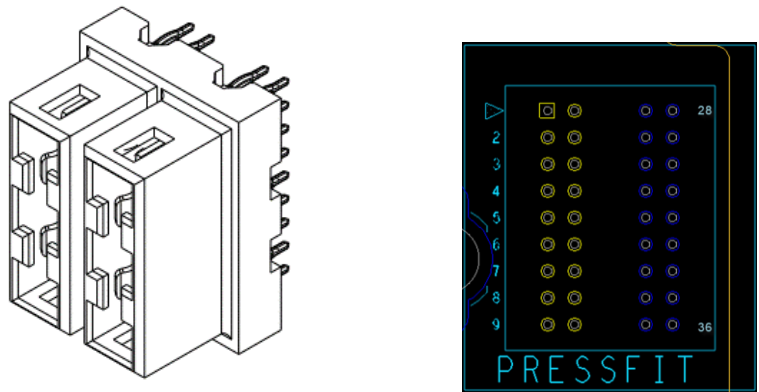
Figure 17 Backplane power connector (HCI) with board layout
