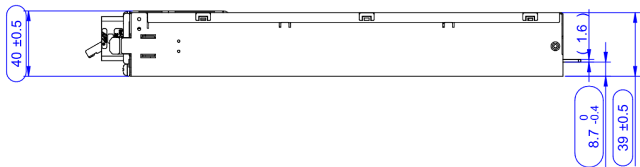
Figure 21 PSU side view
