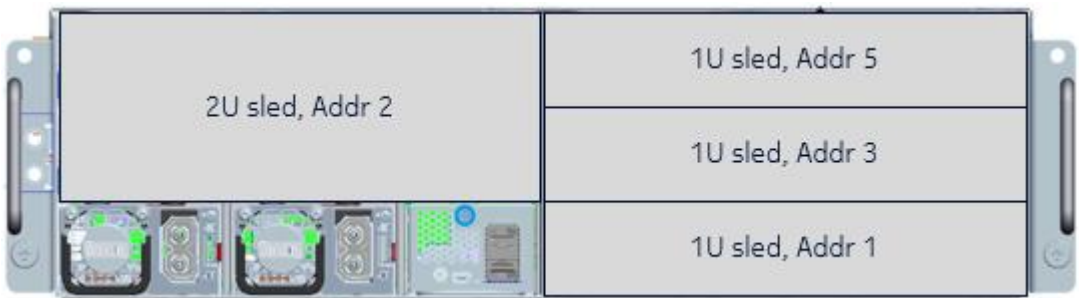
Figure 8 Open edge chassis with three 1U sleds and one 2U sled, option 1
