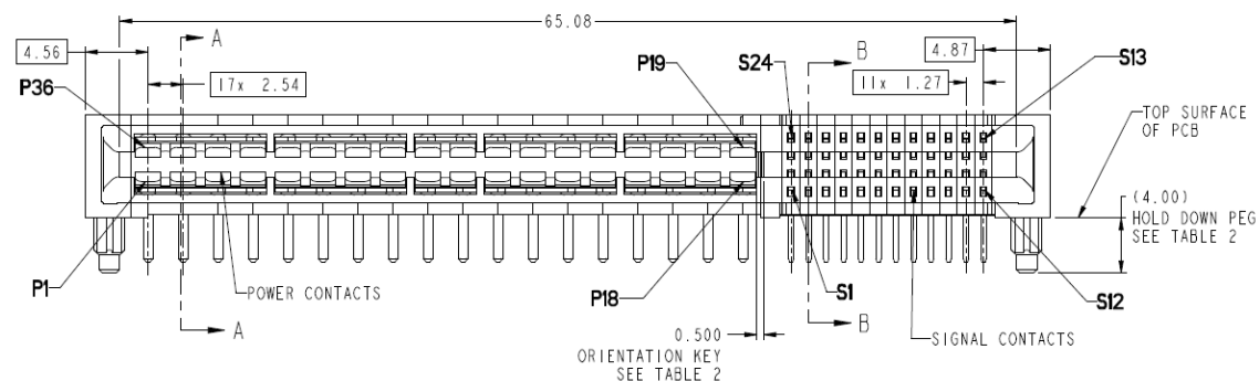
Figure 24 PSU mating connector
