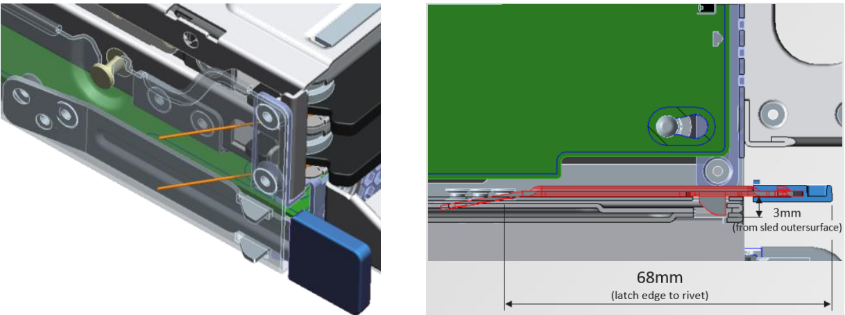
Figure 13 Sled release latch
