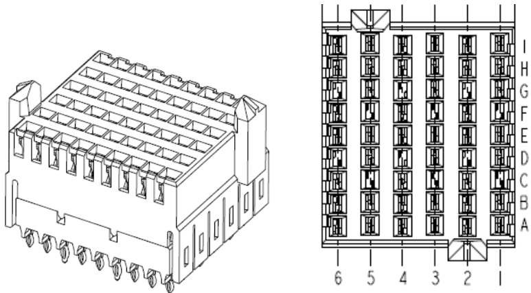
Figure 18 Backplane signal connector with pin map
