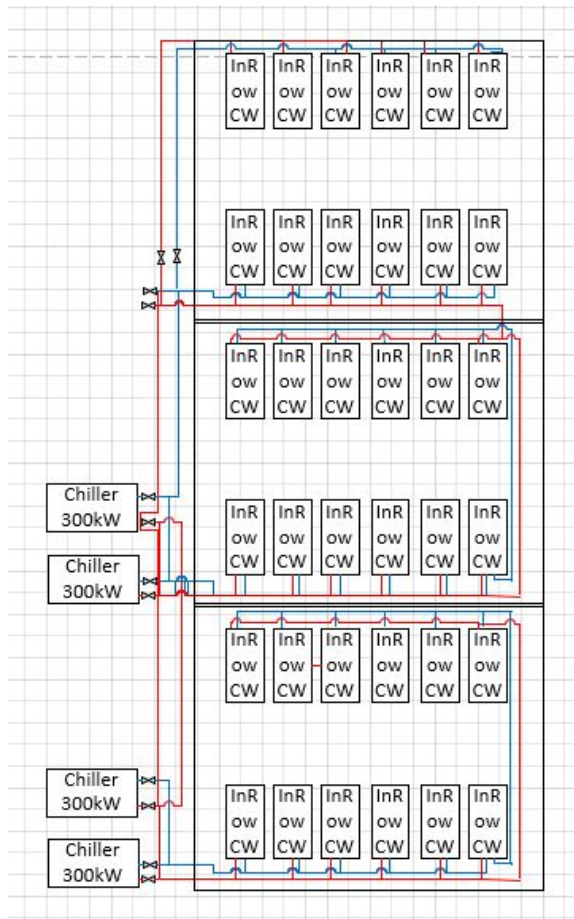
Three modules piping diagram
