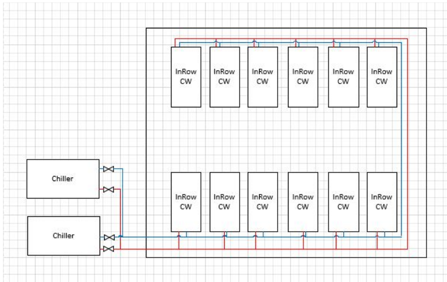
Three modules piping diagram
