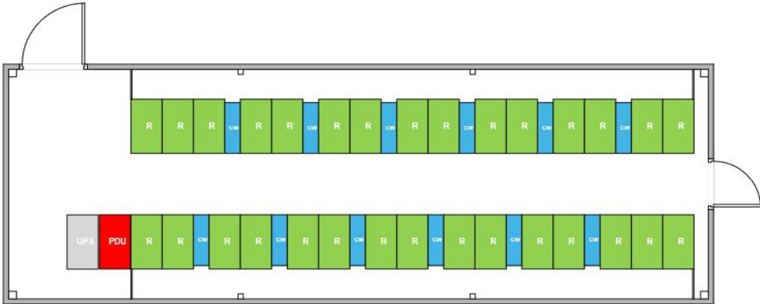
Single module with UPS
