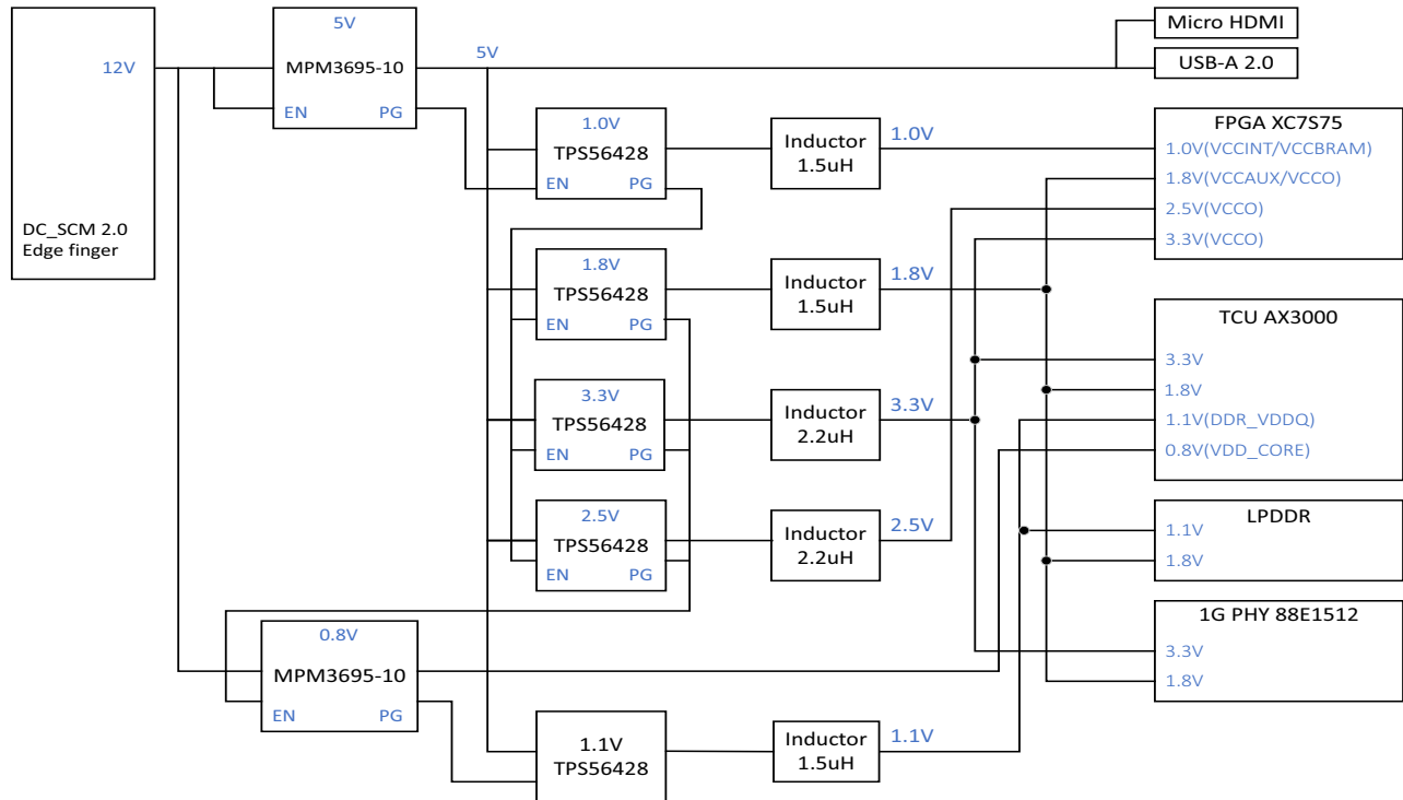
Figure 19. Power Delivery Block Diagram
