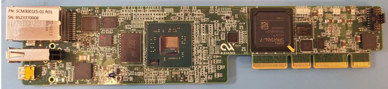
Figure 17. Module Assembly Overview
