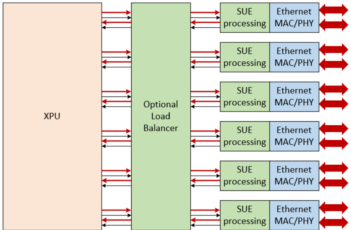
Figure 20 – Example XPU Load Balancer
