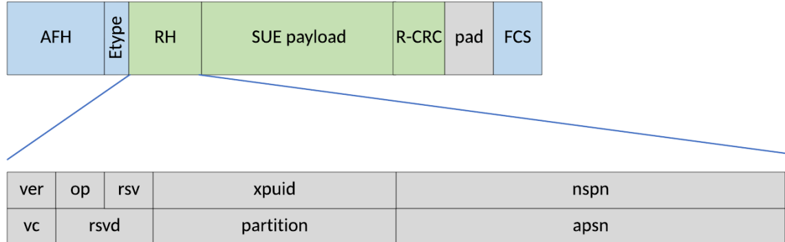
Figure 9 – SUE Reliability Header
