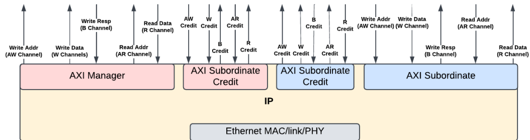
Figure 6 - SUE Datapath AXI Interface
