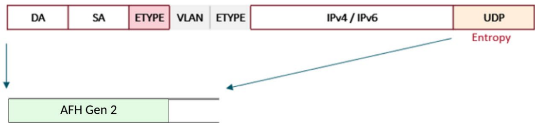
Figure 13 - AFH Gen 2 Header Compression
