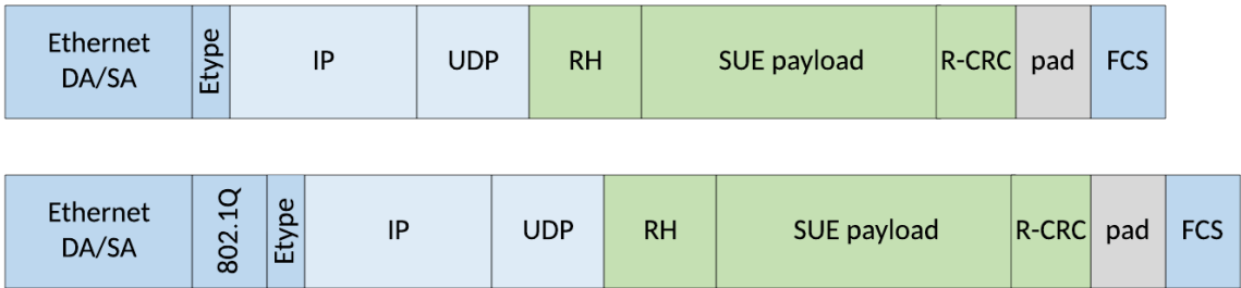
Figure 11 – Standard IEEE 802.3 Ethernet IP Format
