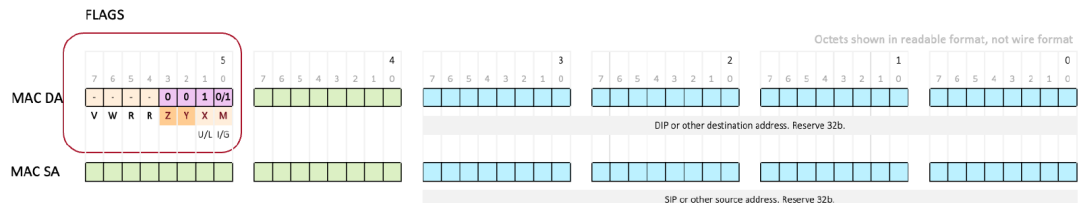
Figure 14 – AFH Gen 2 Field Mapping
