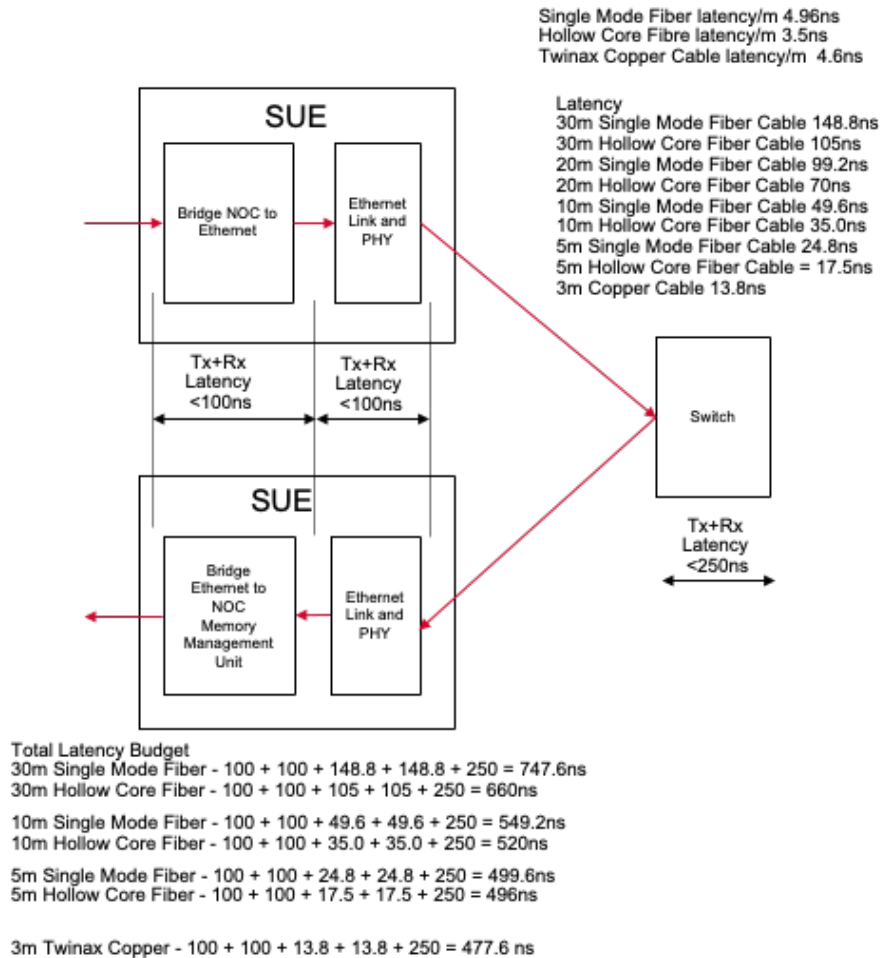
Figure 22 – SUE End to End One Way Latency Budget
