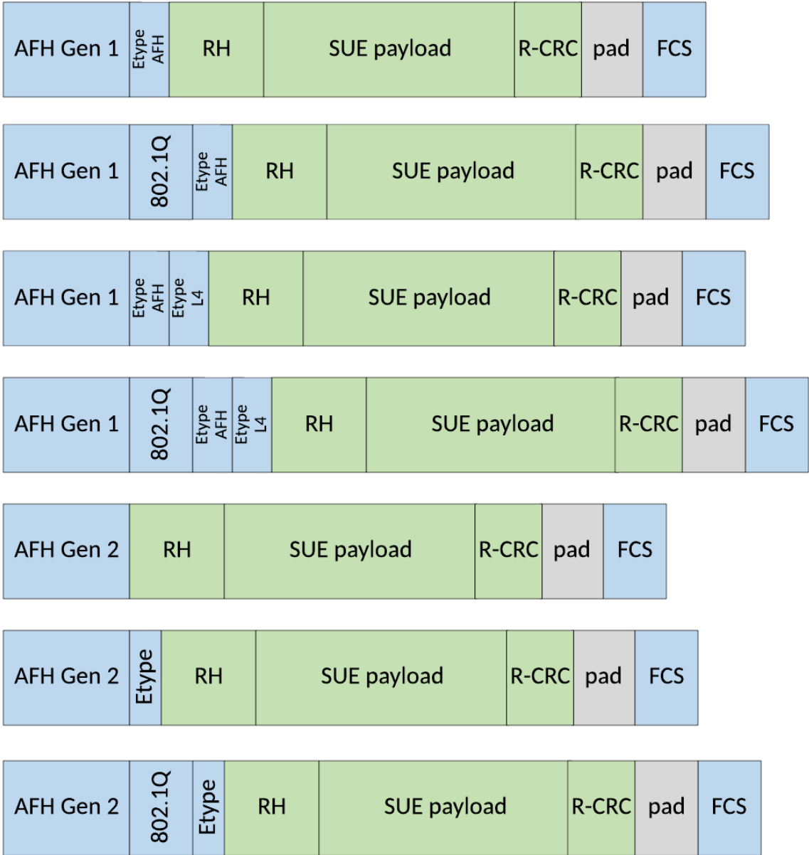
Figure 12 – AFH Gen 1 and Gen 2
