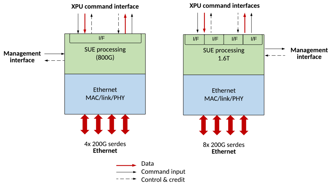
Figure 5 – SUE Interfaces
