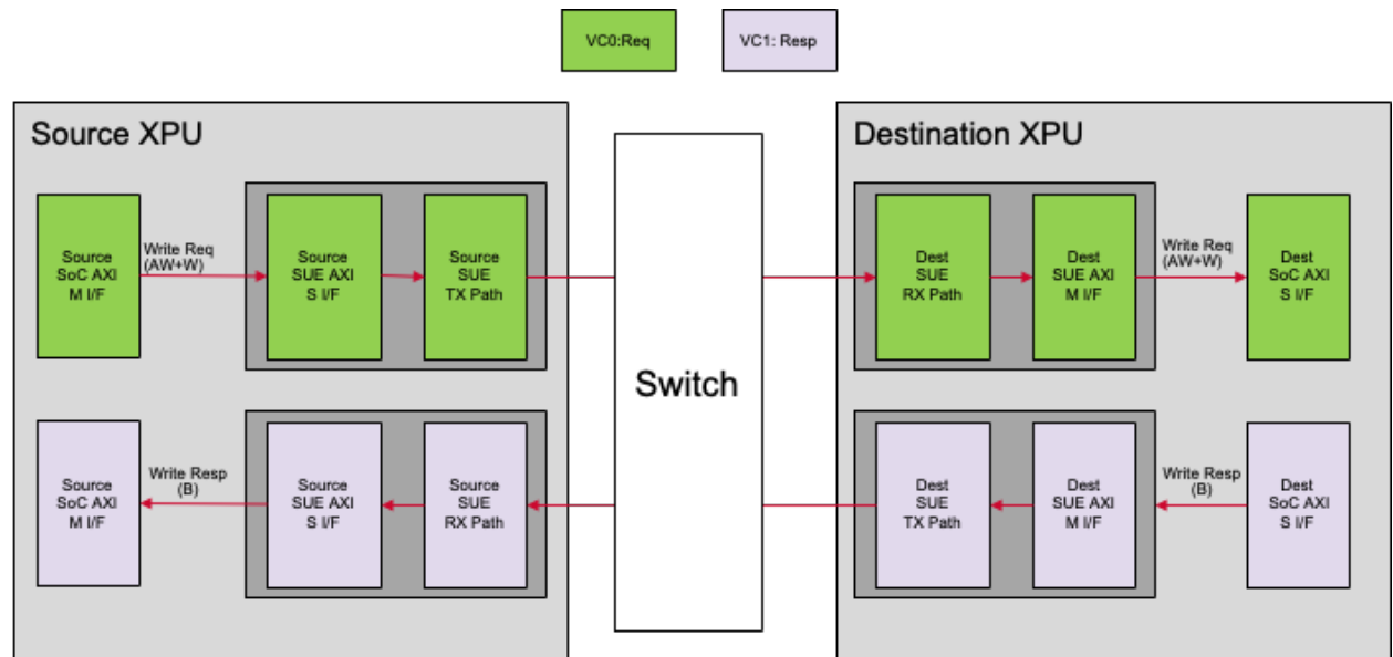
Figure 8 - Datapath AXI interface connectivity (Write/Write Response)
