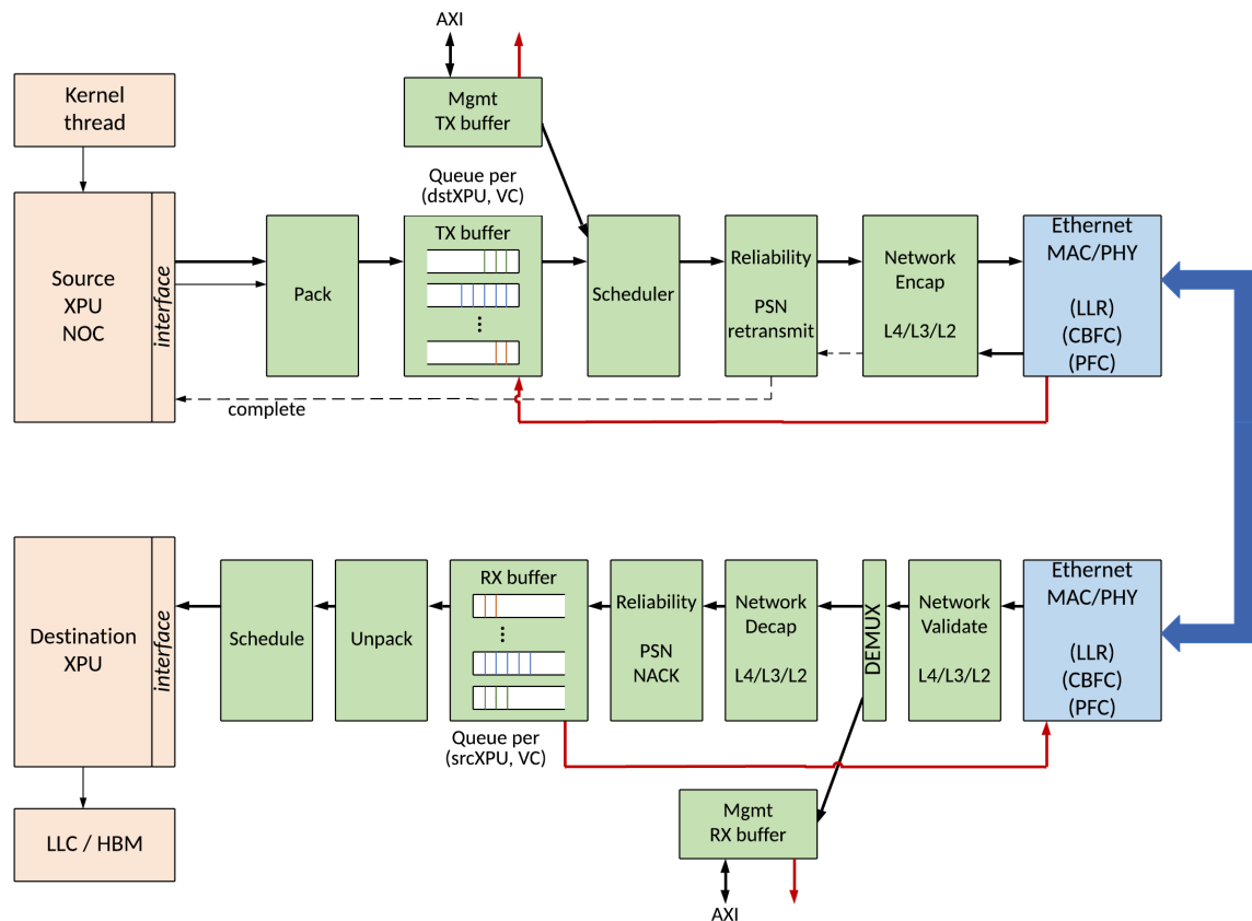
Figure 18 – SUE Processing Flow
