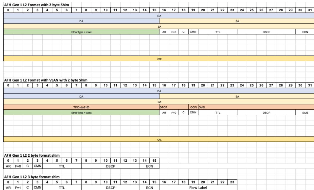
Figure 17 – AFH Gen 1 with Shim Header
