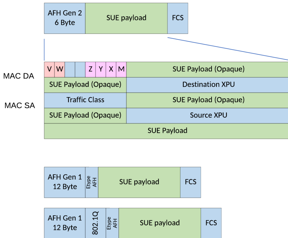
Figure 10 – SUE Lite Encapsulation
