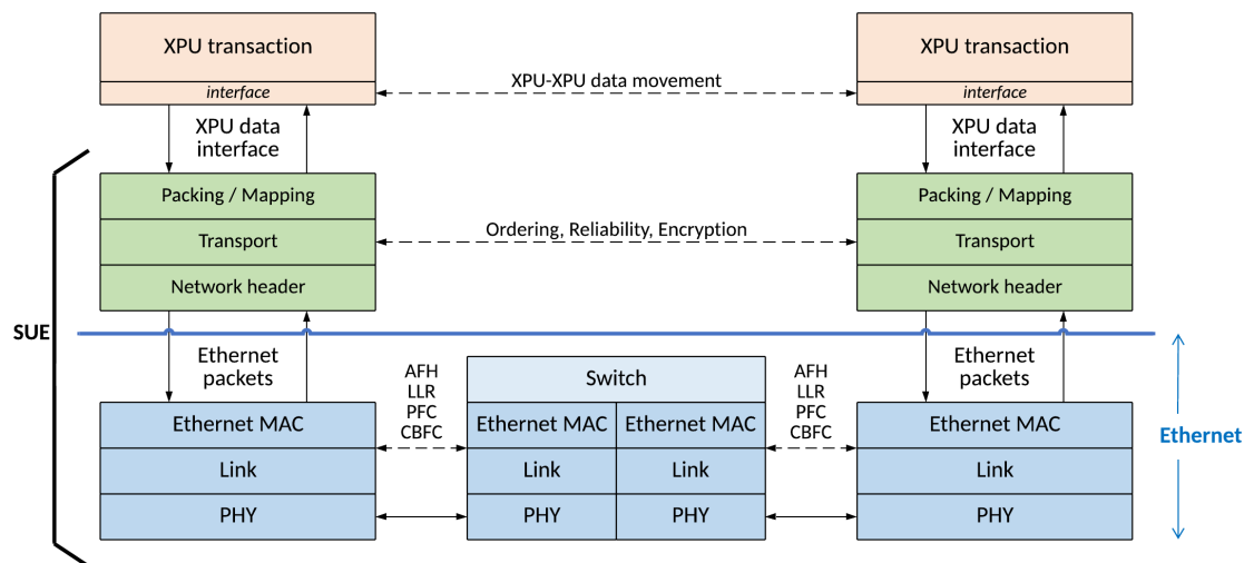
Figure 3 – SUE Stack
