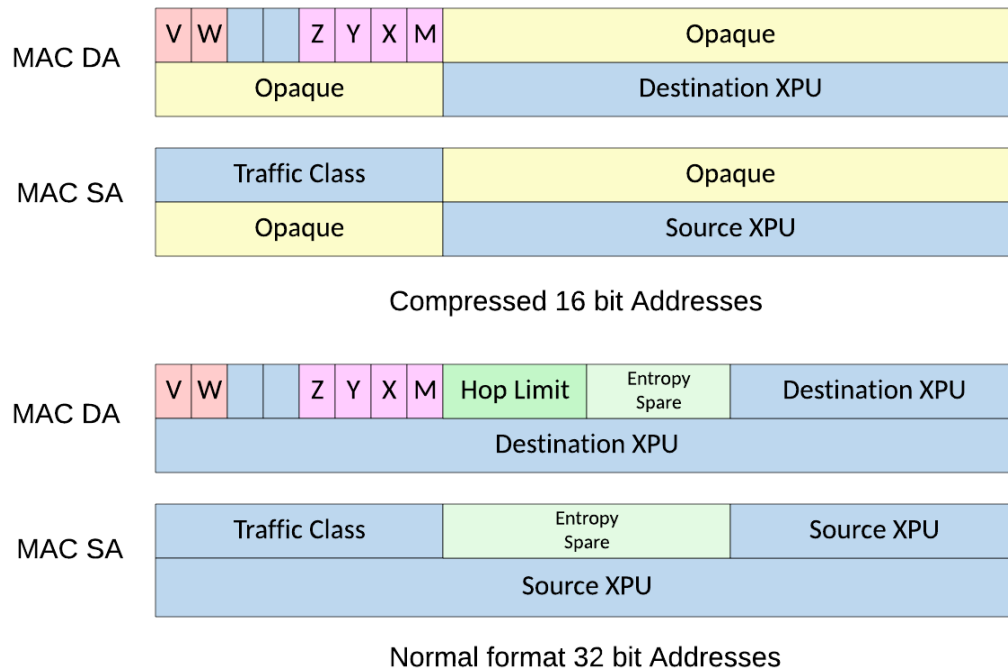
Figure 15 – AFH Gen 2 normal and compressed formats
