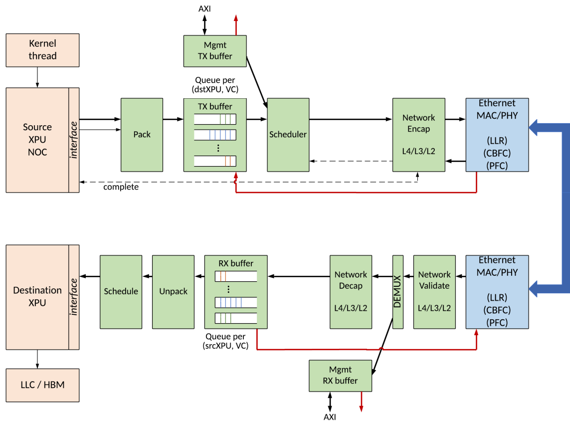
Figure 19 – SUE Lite processing
