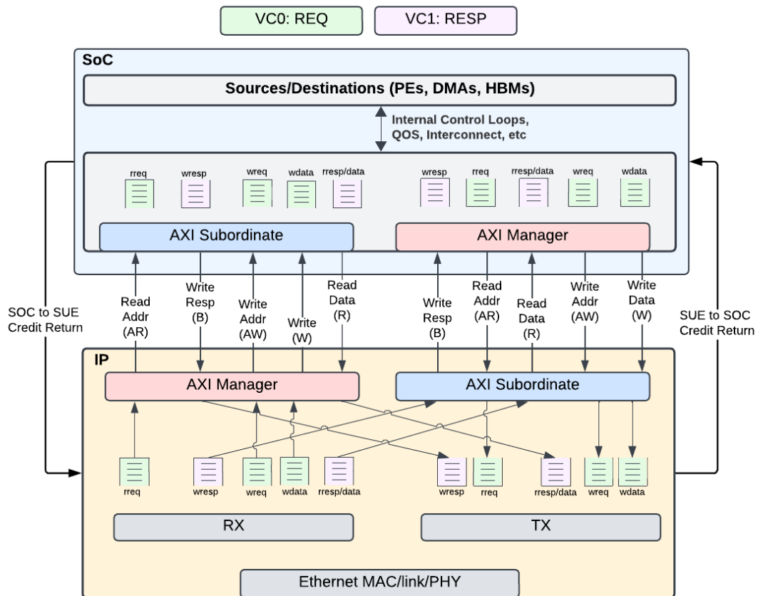
Figure 7 – Datapath AXI interface Connectivity
