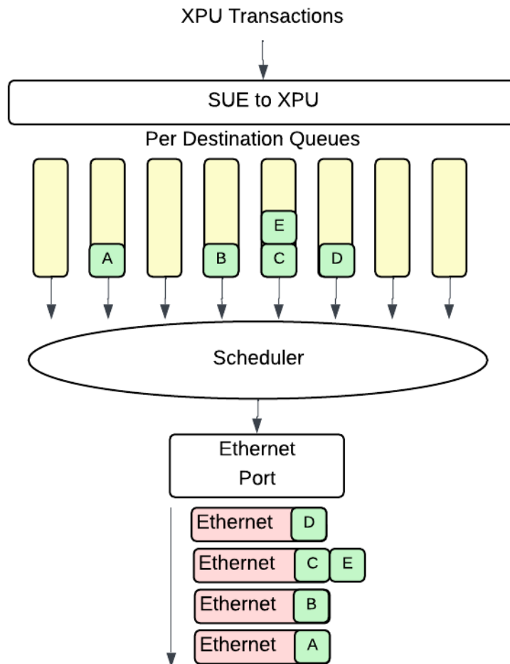
Figure 21 – SUE Packing Example
