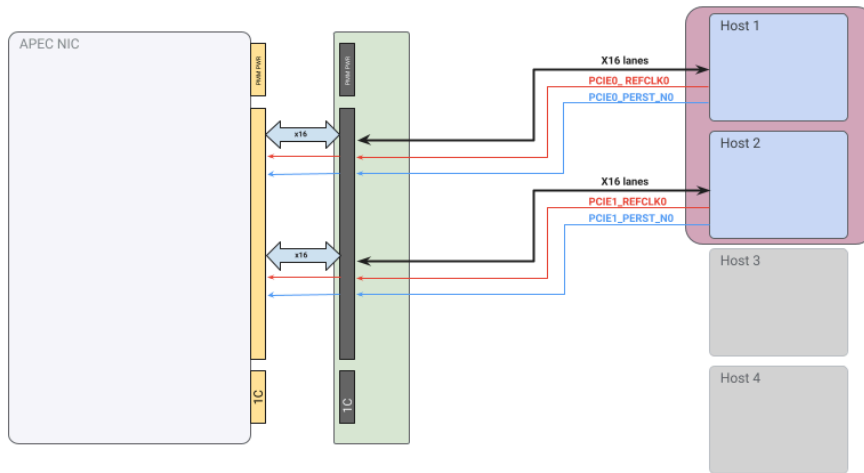
2 x16 Endpoint config - Single chassis
