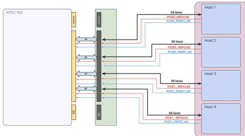
4 x8 Endpoint config - Single chassis concept (No Retimer)
