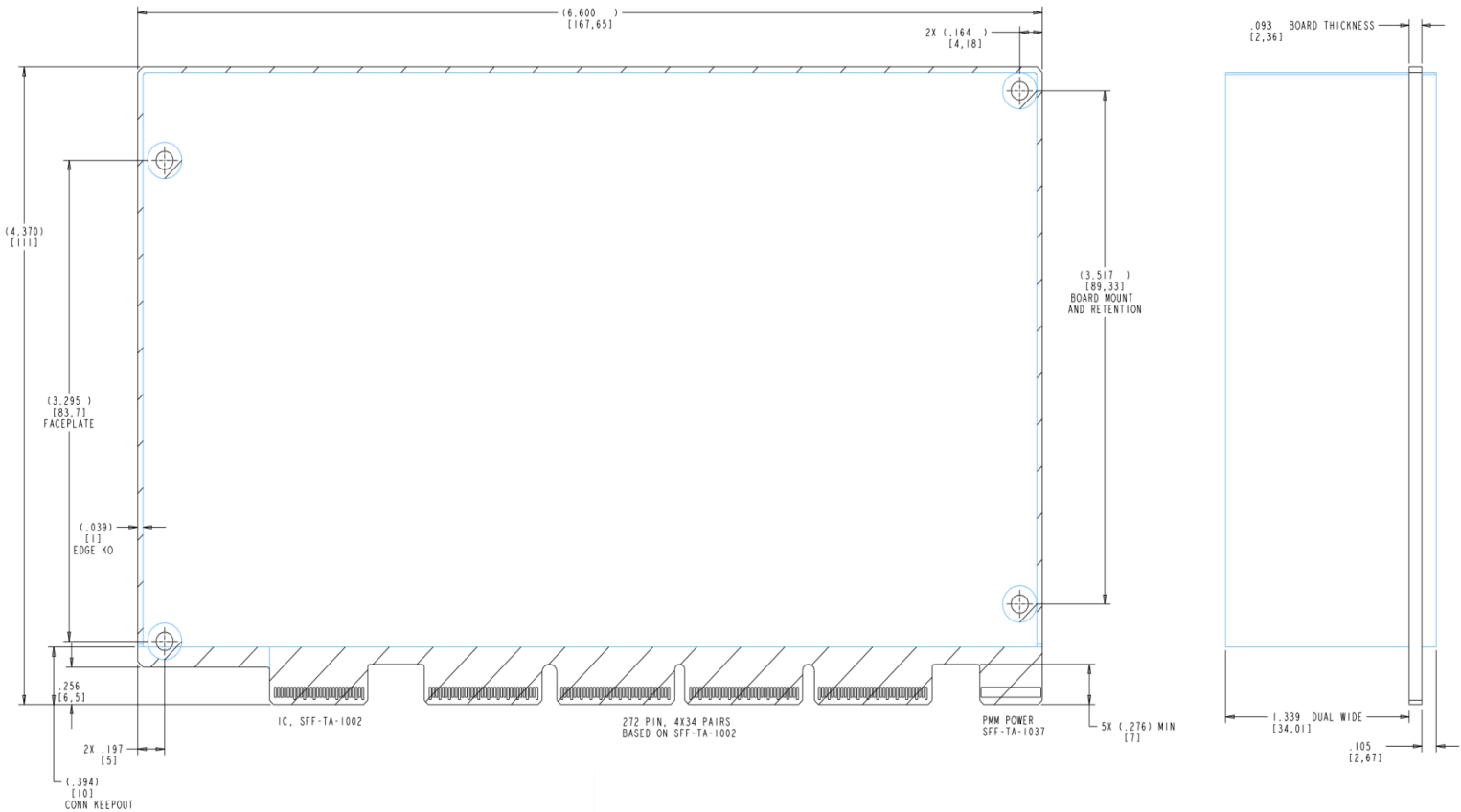
Figure: Board Dimensions
