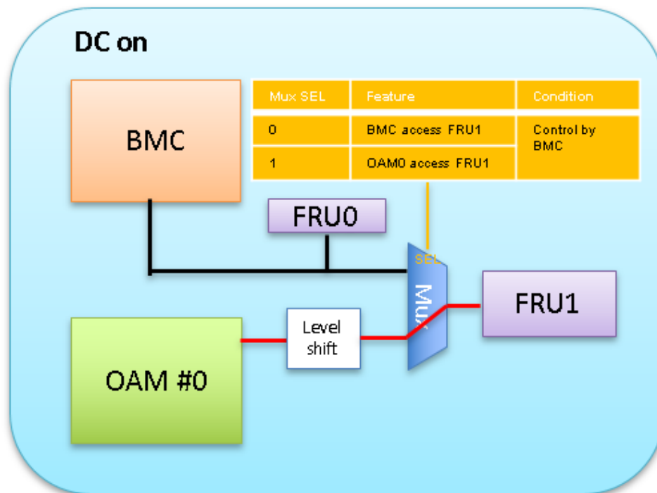
Figure 64 FRU diagram
