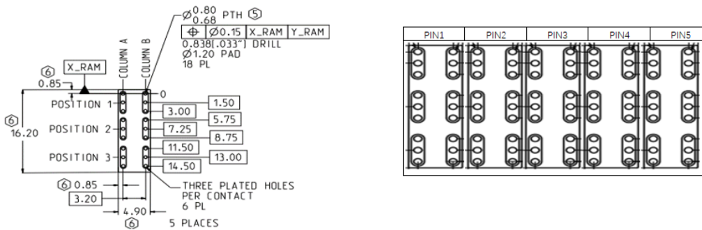
Figure 25 12V power connector pin list
