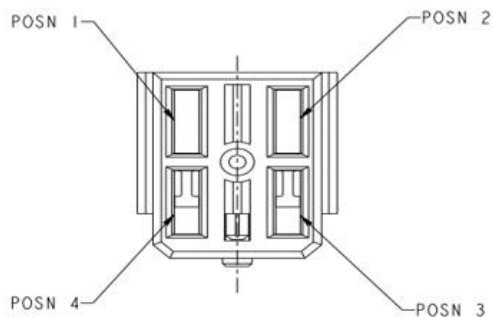
Figure 24 54V power connector
