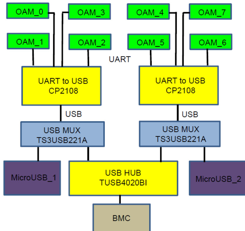
Figure 18 UART Diagram
