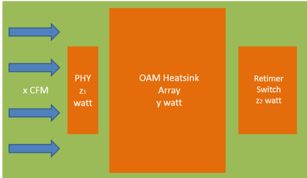
Figure 59 CFM per Watt definition for UBB
