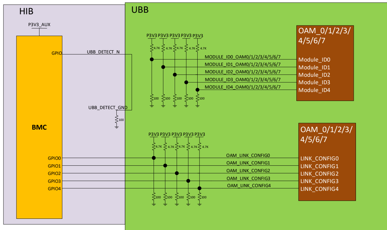
Figure 31 LINK_CONFIG ID
