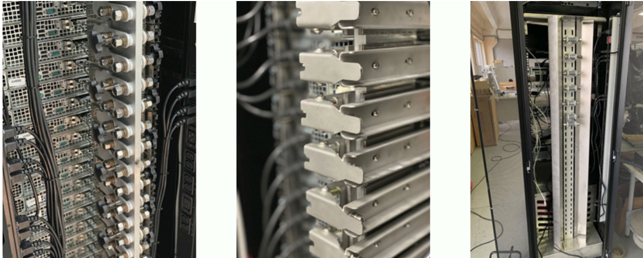
Figure 8: Dry (Mechanical) Quick Disconnect 6
