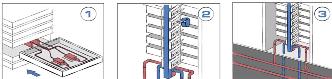
Figure 6: Image to show dry quick disconnect system
