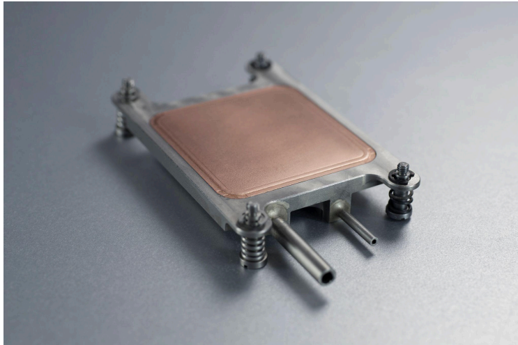
Figure 3: Example of an LHP Evaporator 3
