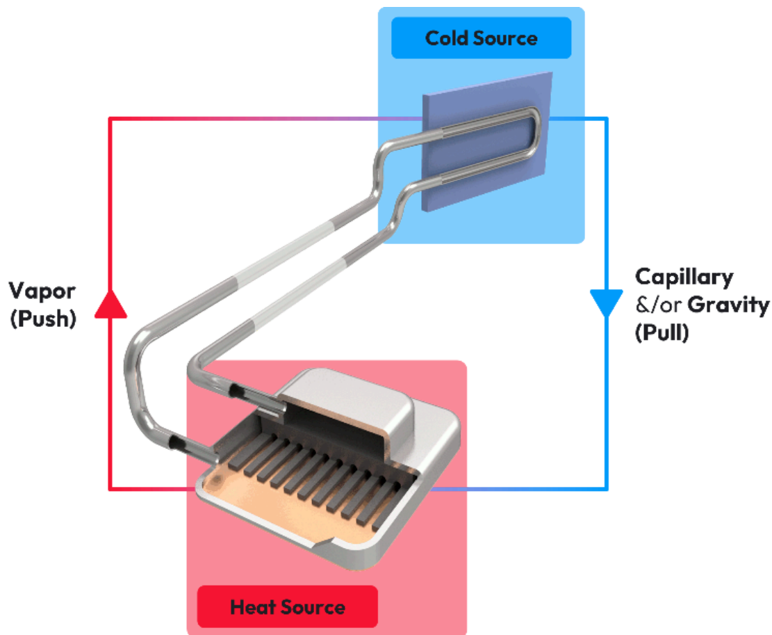
Figure 2: LHP Operating Diagram 3
