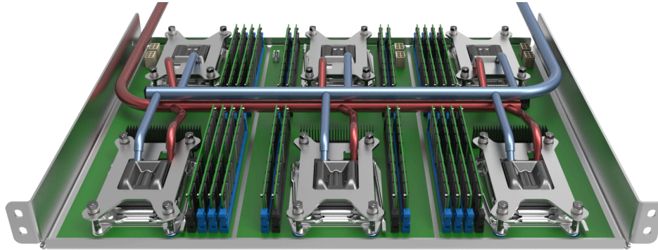
Figure 4: Representative parallel multiple cold plate configuration
