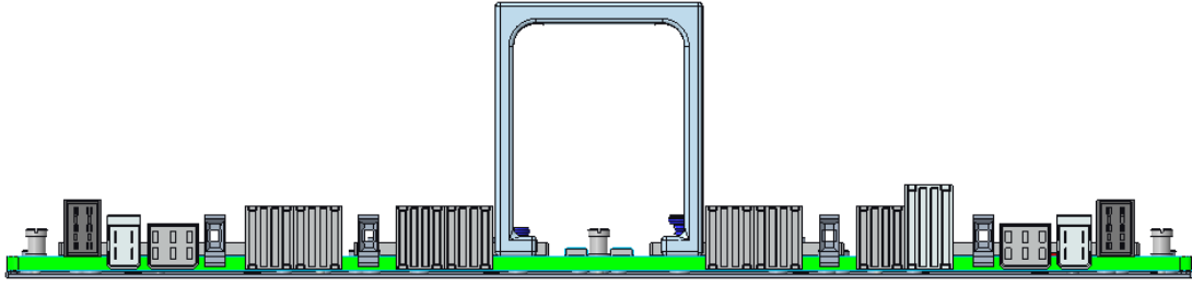
Figure 45 UBB high speed and power connectors to HIB
