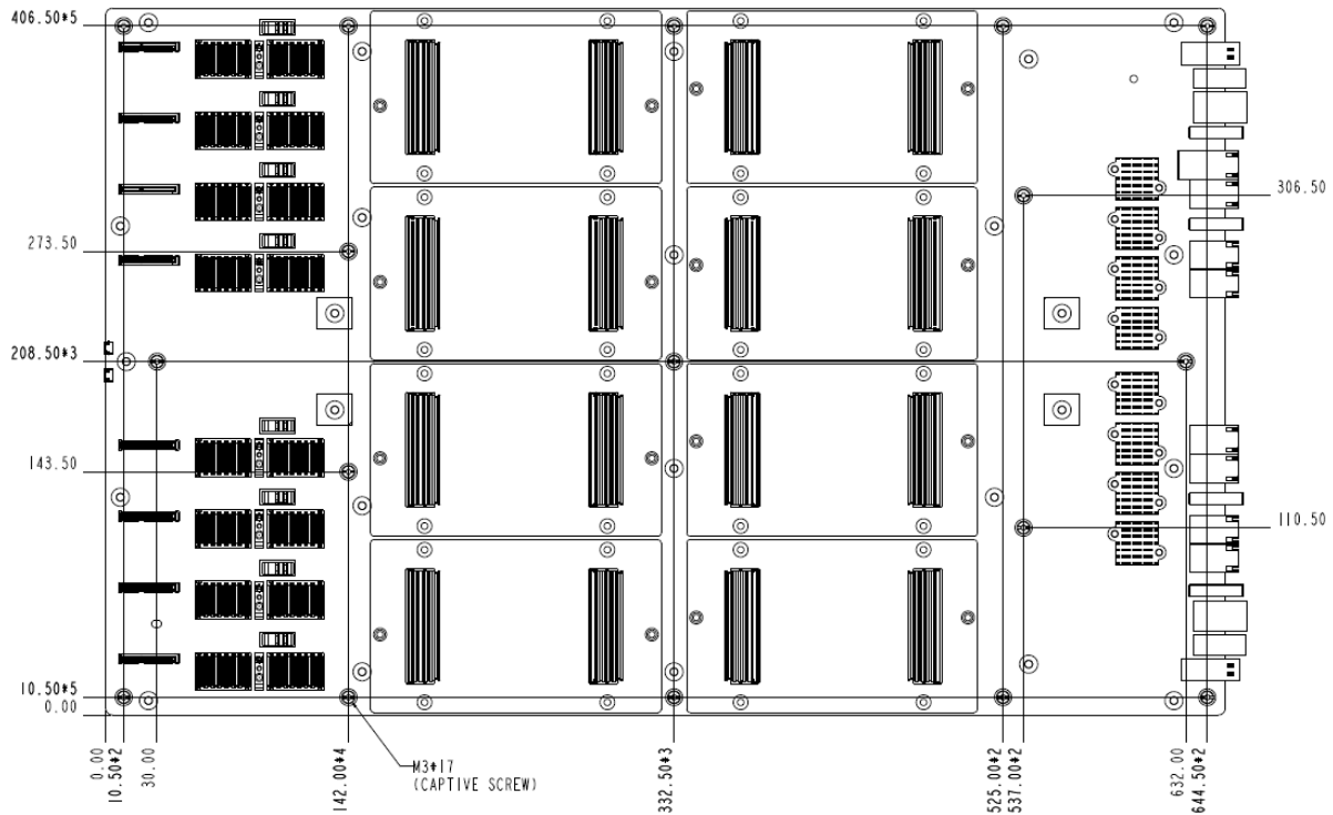
Figure 47 mounting holes
