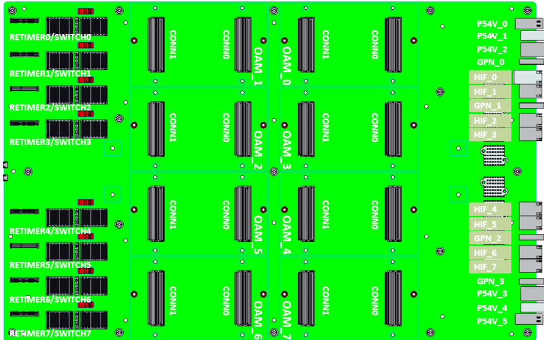
Figure 39 UBB silkscreen example
