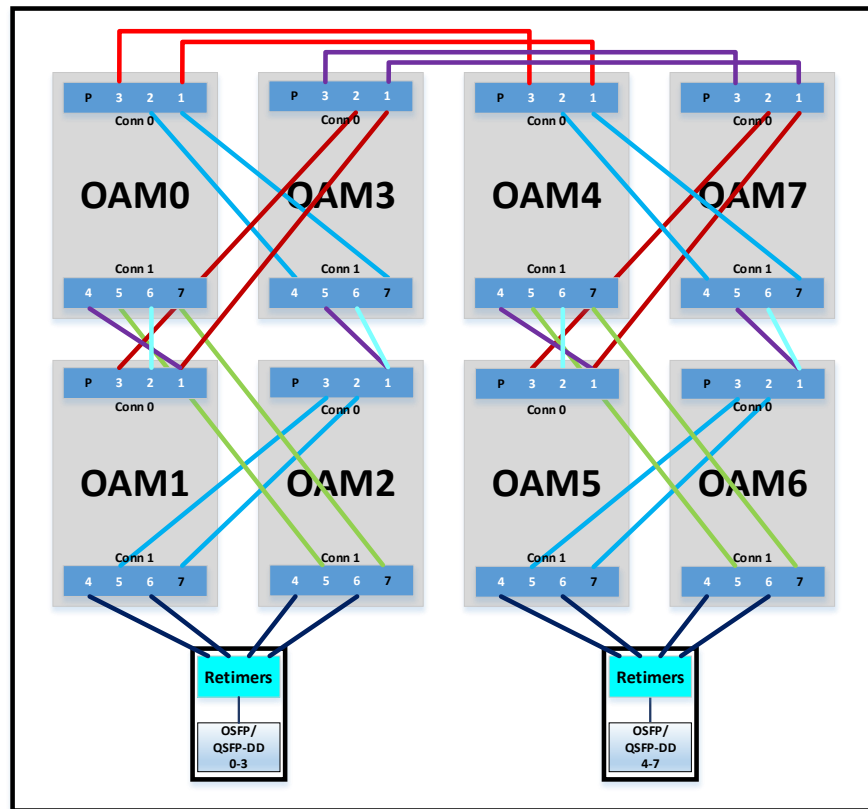
Figure 30 8-port HCM topology routing guide
