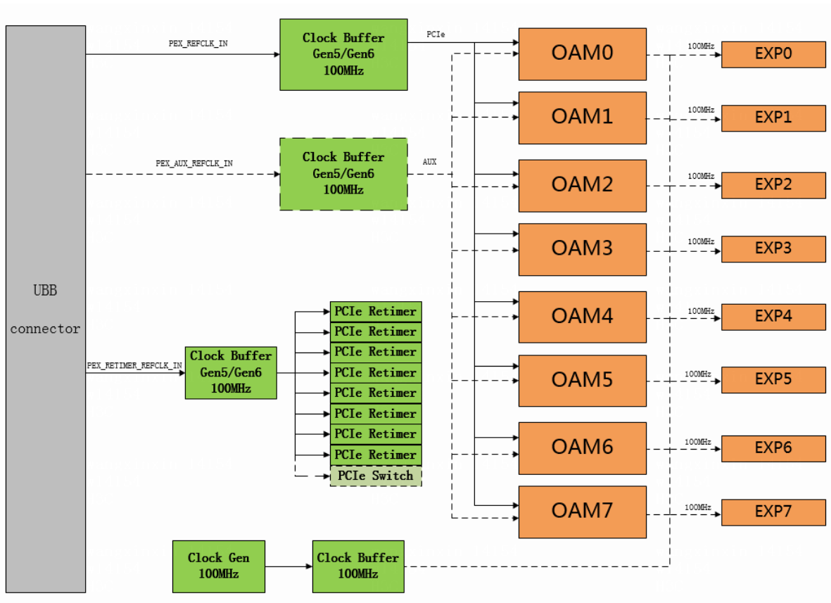
Figure 11 OAI Reference UBB clock diagram
