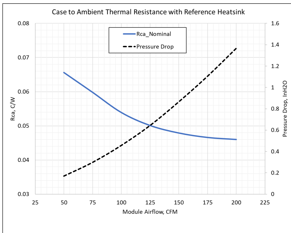
Figure 62 Reference OAM Heatsink with 3D-VC technology
