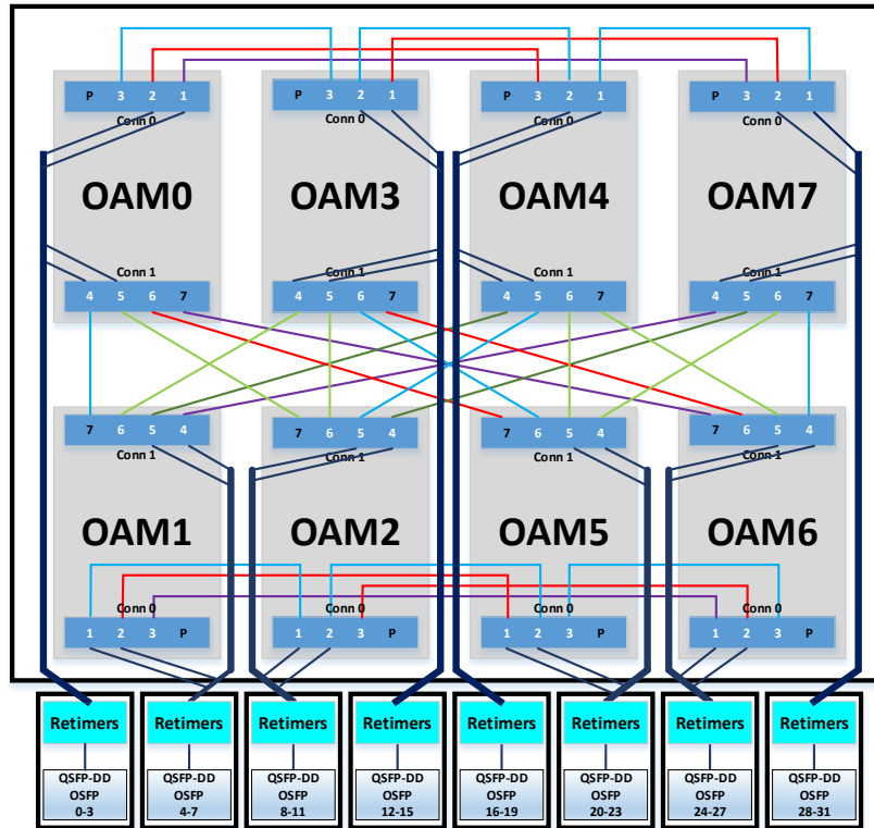
Figure 37 11-Port (7+4) FC/Retimer Topology
