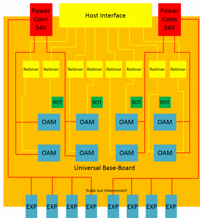
Figure 4 Example of UBB System Building Blocks
