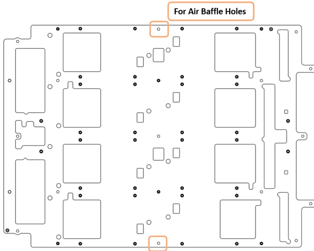
Figure 51 Air Baffle mounting holes on the stiffener
