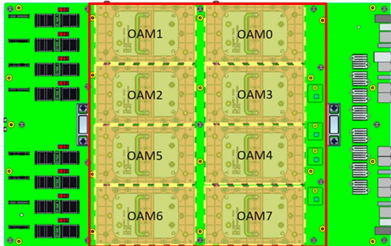
Figure 58 UBB heatsink recommended airflow area keep out
