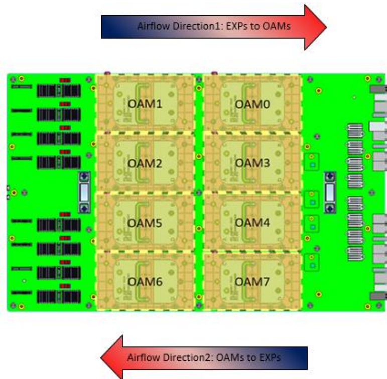
Figure 57 UBB at different airflow directions
