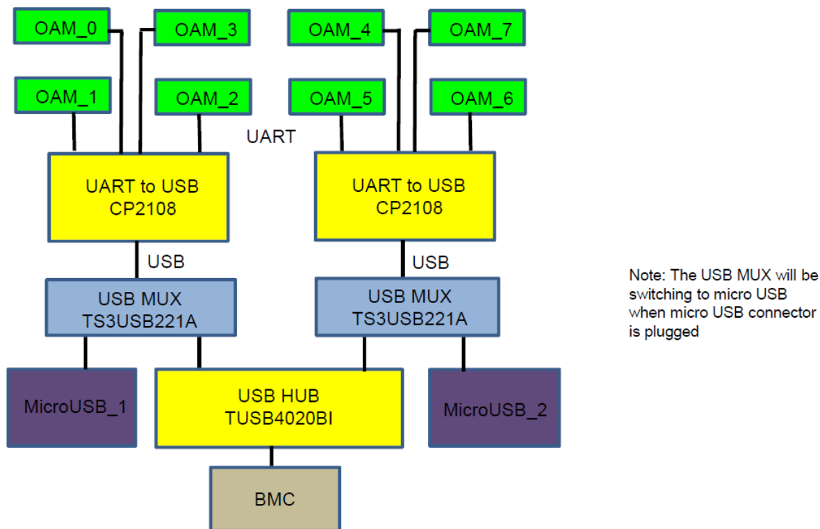
Figure 18 UART Diagram
