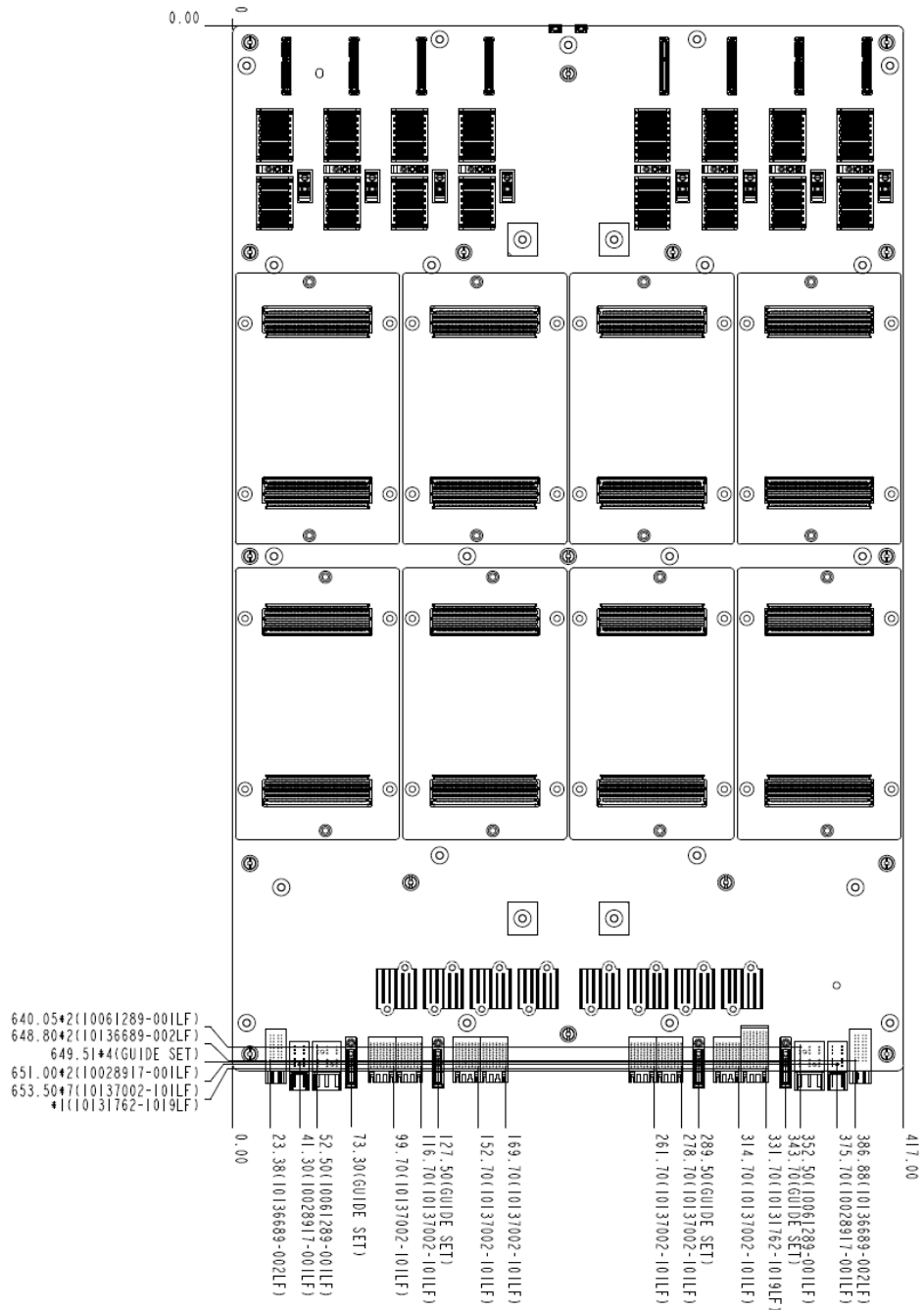
Figure 46 UBB high speed and power connectors coordinate
