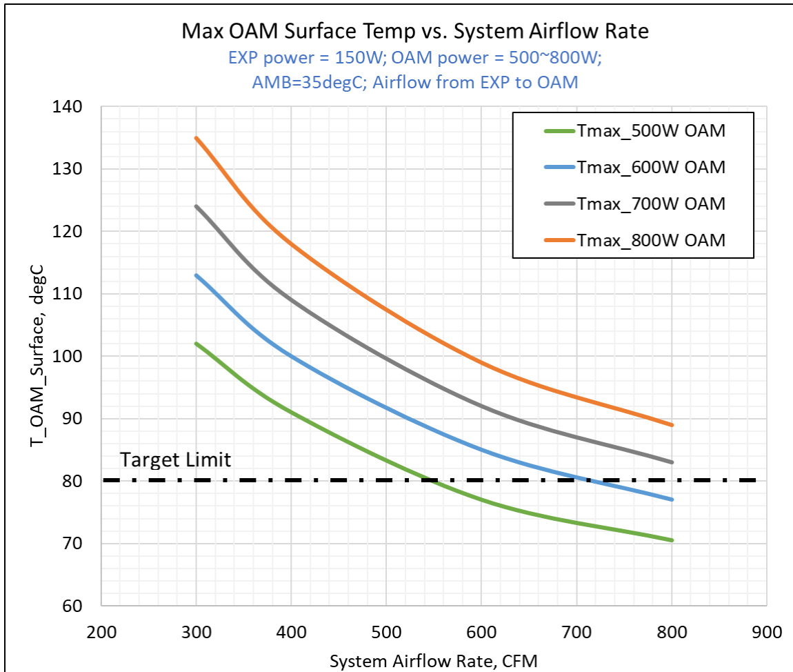
Figure 64 Max surface temperature of hottest OAM in the UBB2.0 system, at AMB = 35degC, sea level, airflow direction EXP-to-OAM, with various airflow rates and OAM power. Many assumptions apply to this analysis.
