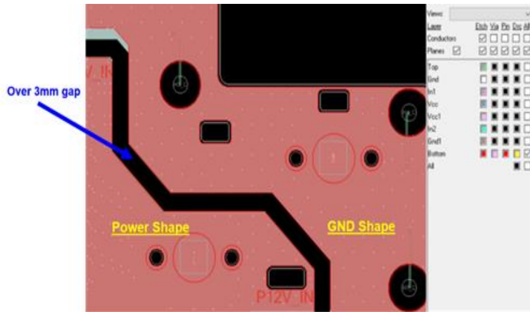
Figure 10 power and GND isolation
