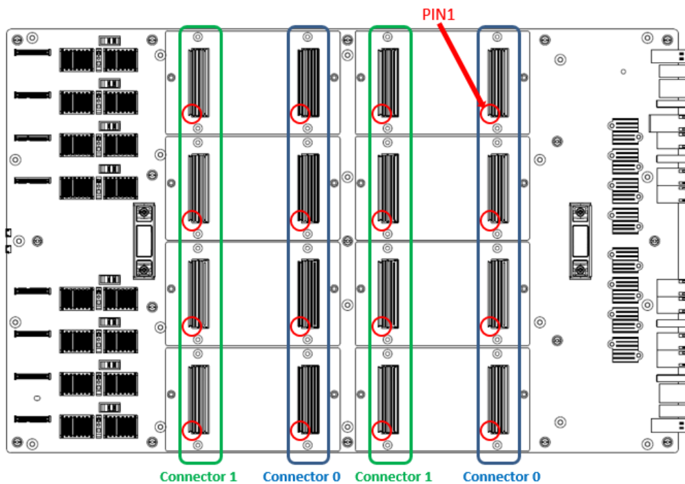
Figure 31 OAM Mirror Mezz Pro connector pin1 HCM orientation
