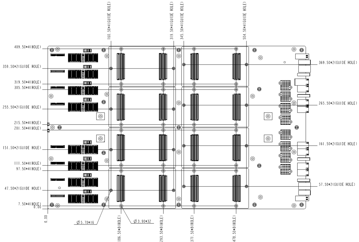
Figure 48 OAM through holes
