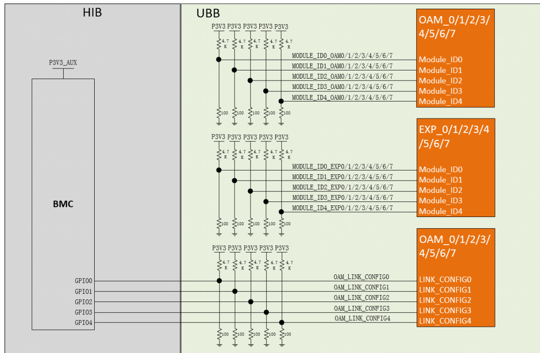
Figure 25 LINK_CONFIG ID
