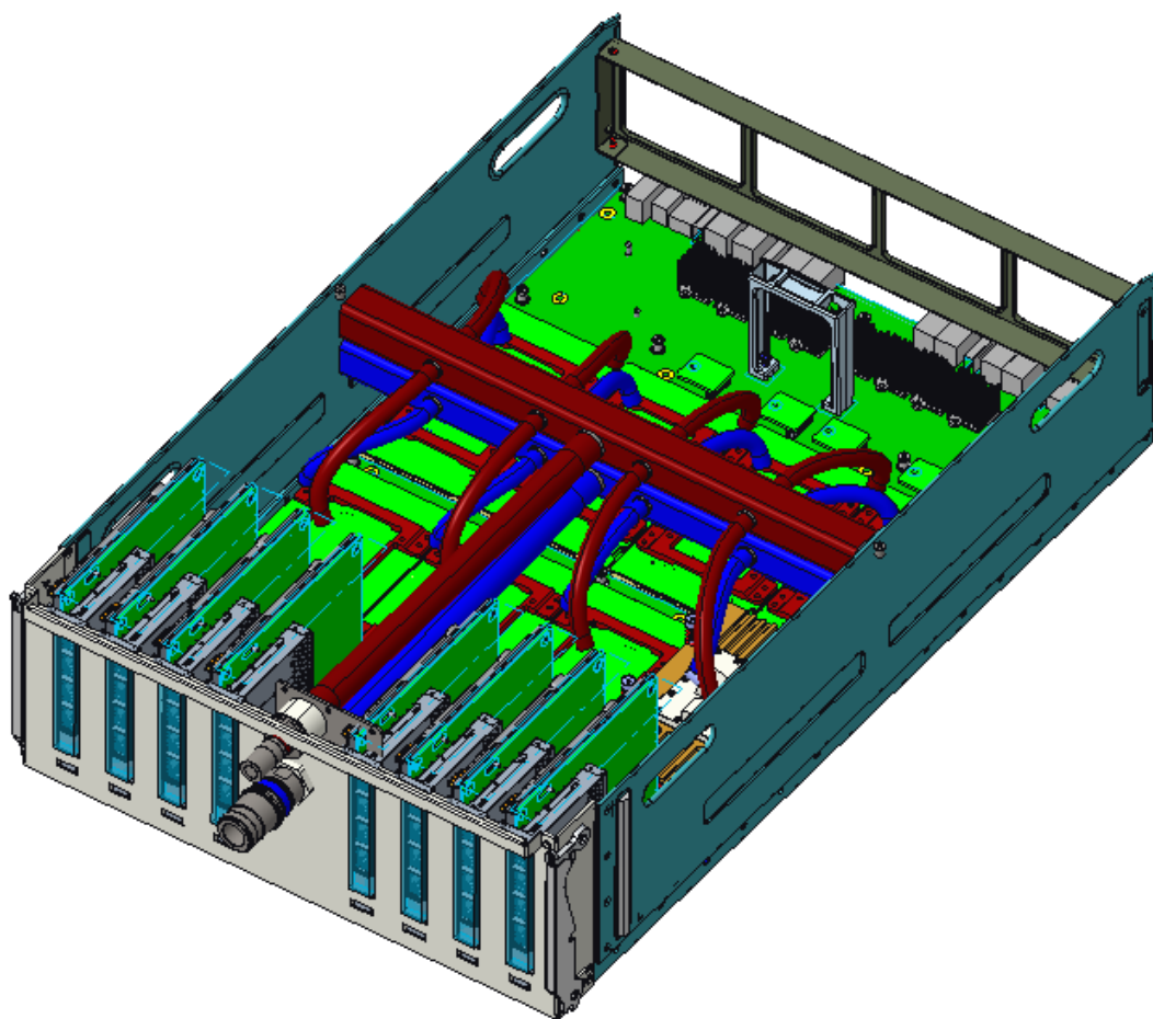
Figure 65 Reference Liquid Cooling Design for UBB. 1: Universal Base Board; 2: Host Interface Board; 3: Power Distribution Board; 4: Liquid Cooling Module. The cooling components and OAMs in the figure are just for concept demonstration and do not represent real solutions.
