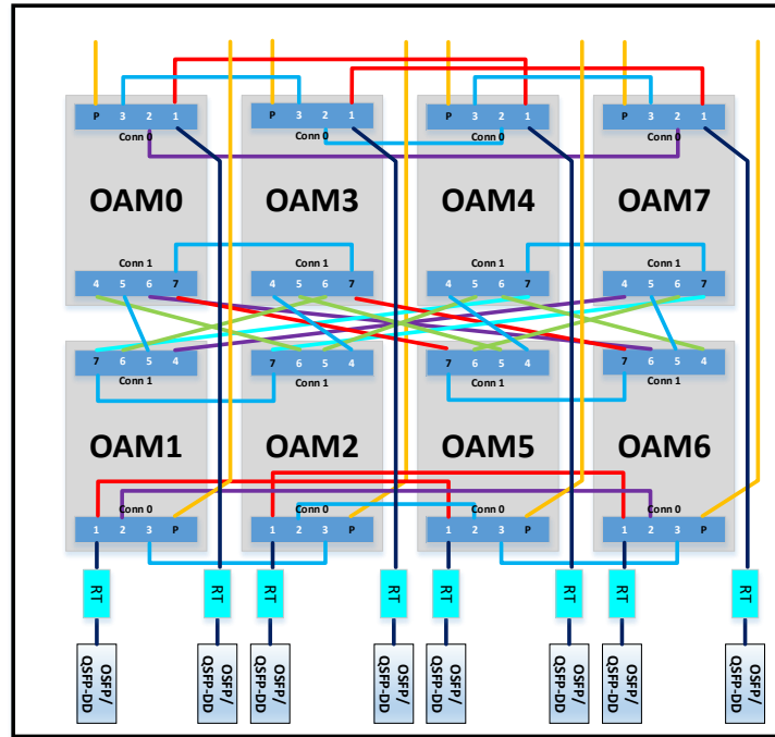
Figure 27 Detail port mapping and routing guidance
