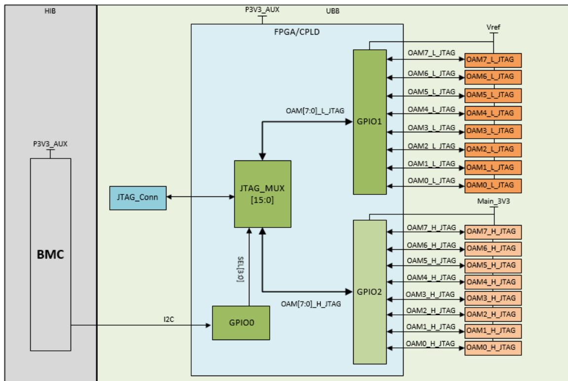
Figure 17 JTAG diagram
