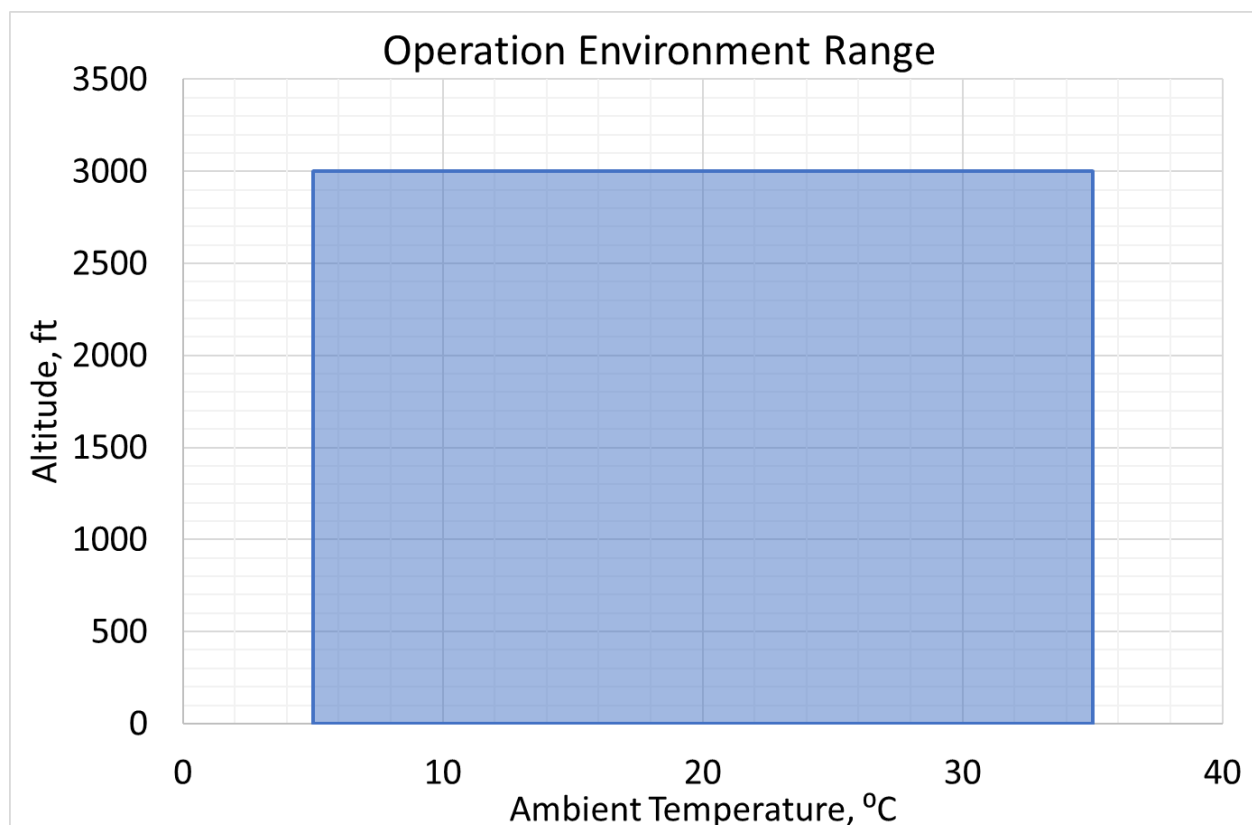
Figure 56 Module Operation Ambient Temperature
