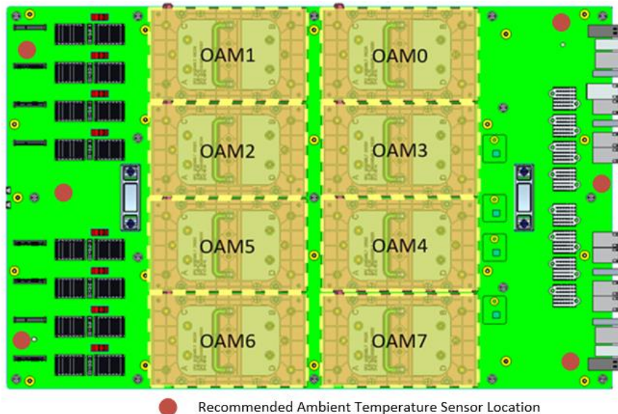
Figure 60 Recommended Ambient Temperature Sensor Map
