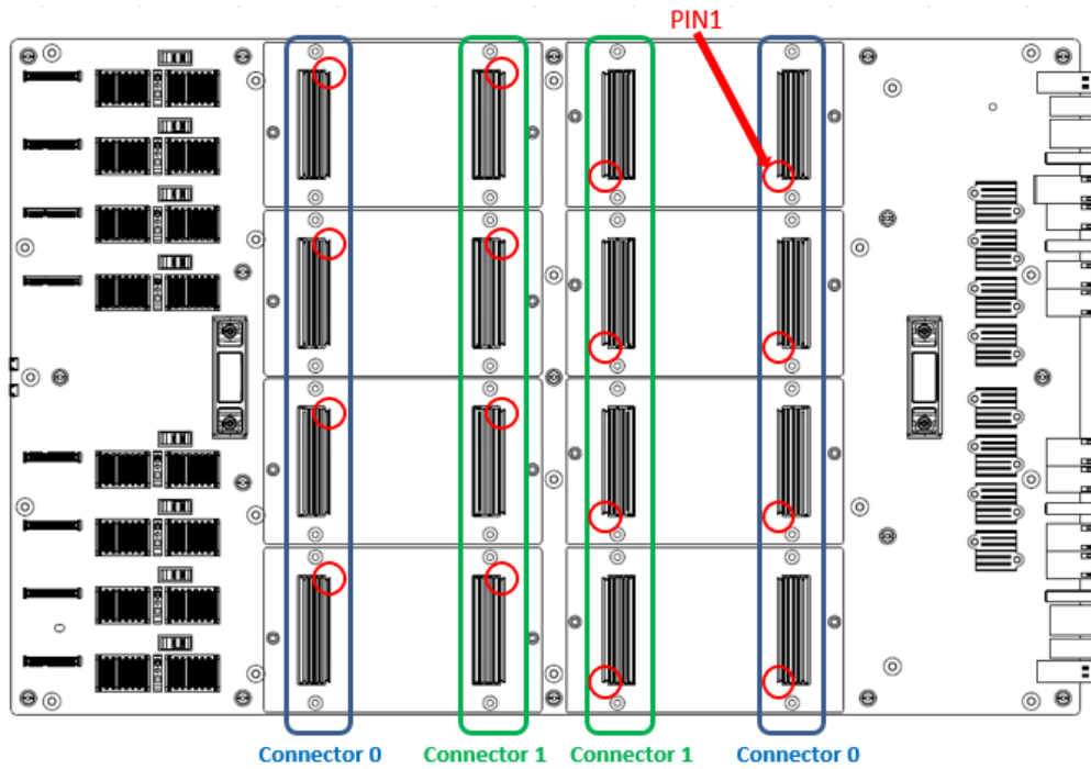
Figure 42 OAM Mirror Mezz Pro connector pin1 FC orientation
