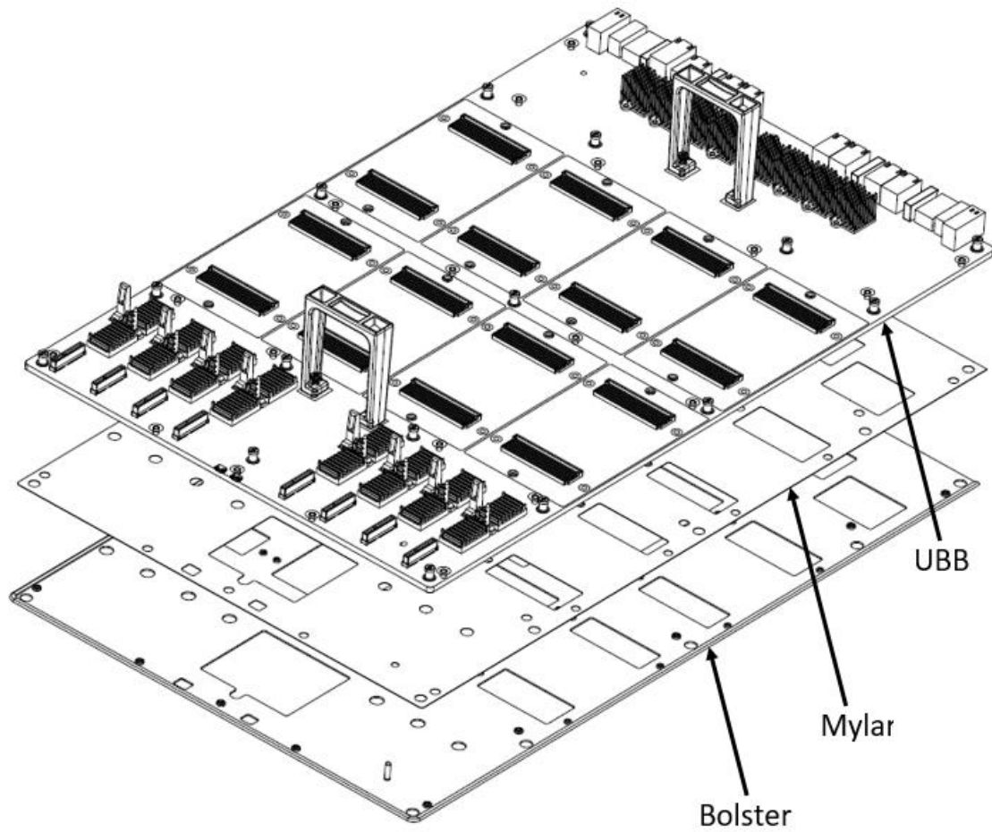
Figure 53 UBB assembly DWG
