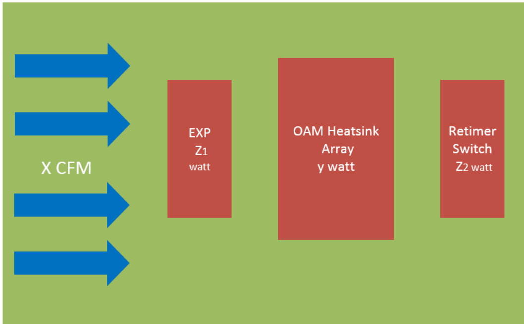
Figure 61 CFM per Watt definition for UBB
