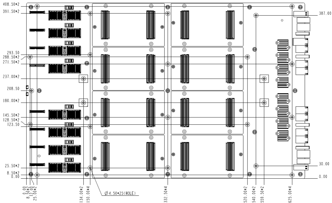
Figure 50 Mounting holes for bolster
