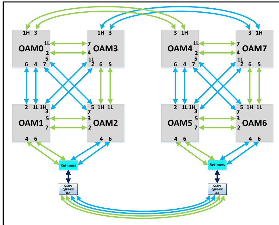
Figure 29 8-port Hybrid Cube Mesh Topology
