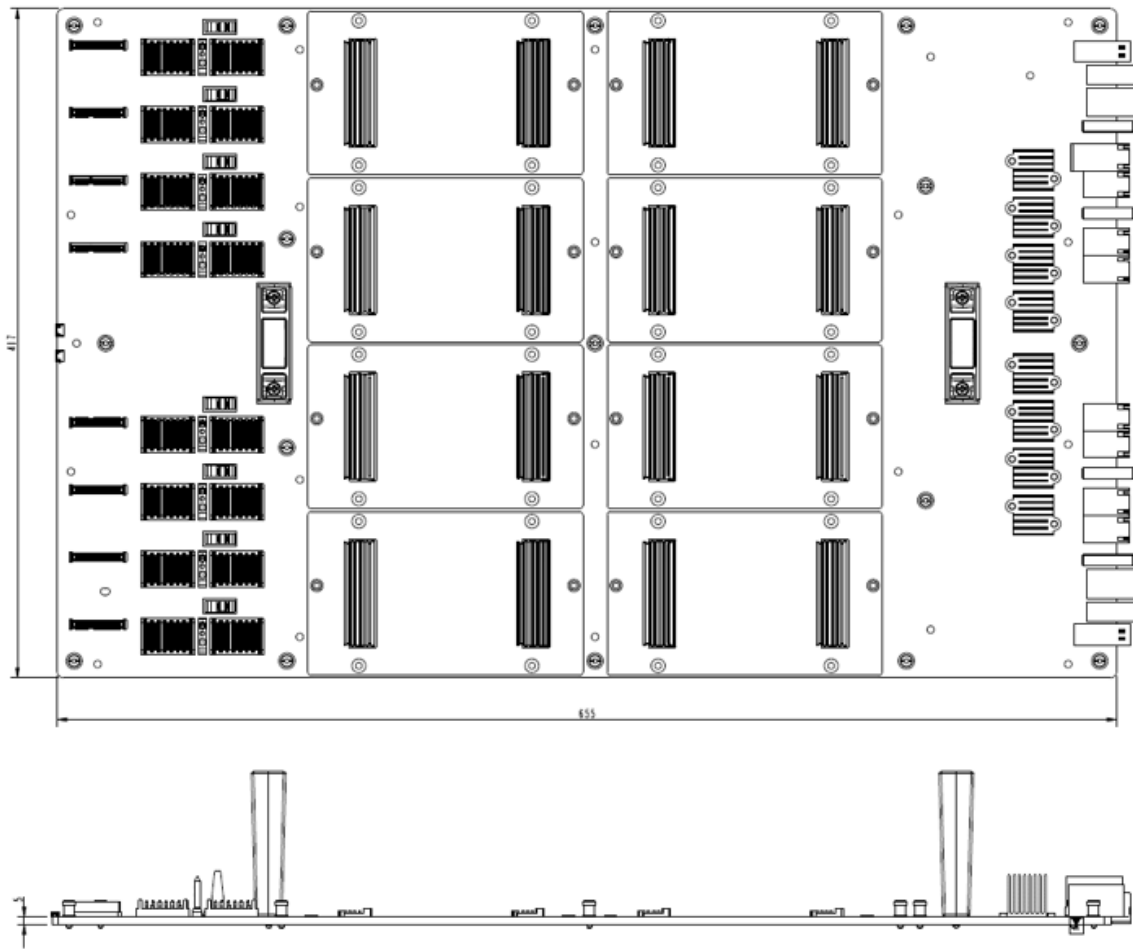
Figure 41 UBB board Top and side views
