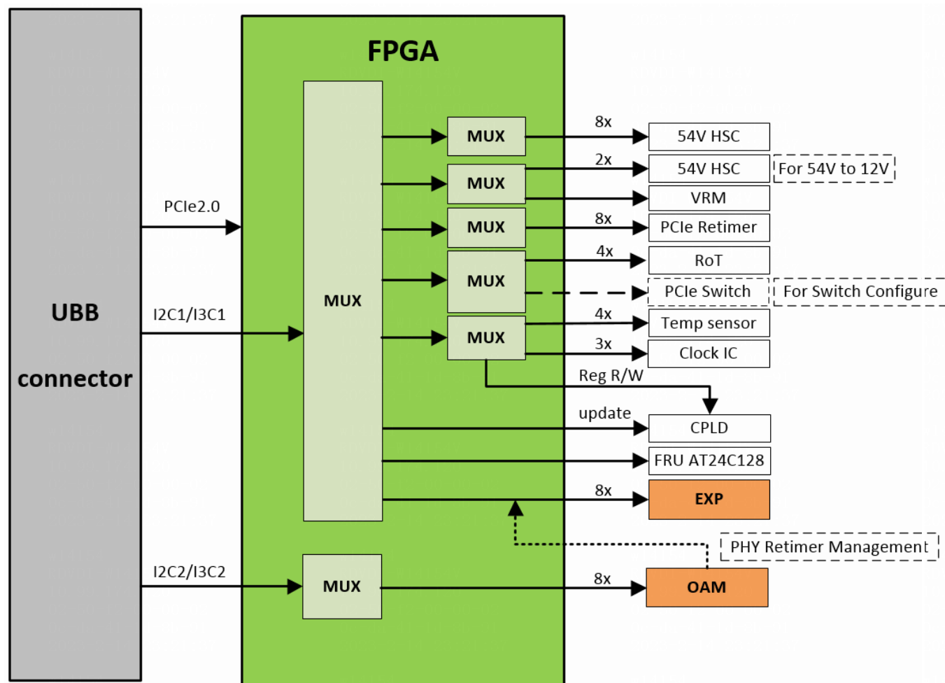
Figure 66 UBB I2C Topology
