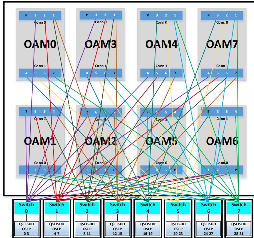
Figure 38 8-port Switch-Based Topology
