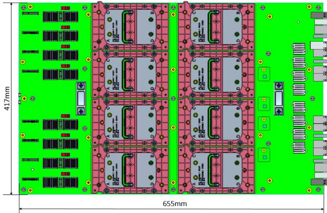
Figure 40 UBB board dimension
