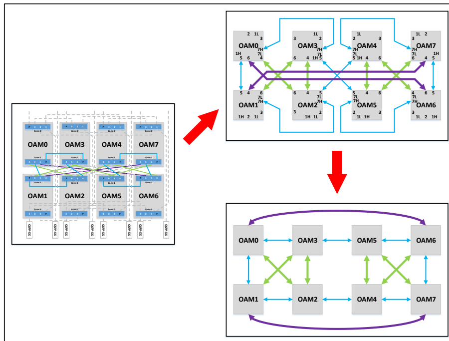
Figure 28 Embedded HCM Topology
