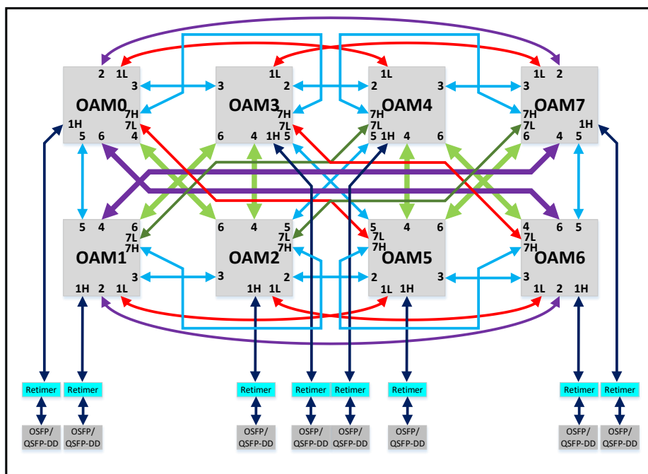
Figure 26 Combined FC/6-Port HCM Topology
