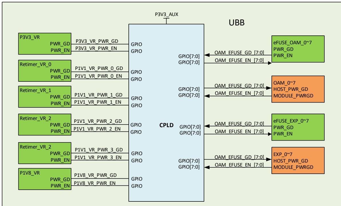
Figure 14 Power Control Block Diagram
