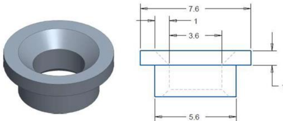
Figure 49 OAM guide hole
