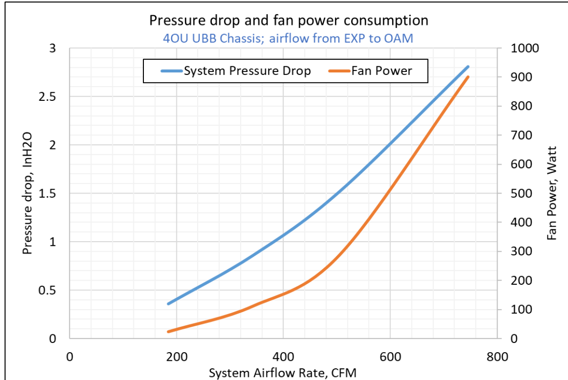
Figure 63 CFD model of the reference 4OU UBB2.0-based platform; pressure drop and fan power consumption for various airflow rates
