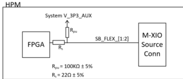
Figure 9: SB_FLEX[1:2] Default Configuration
