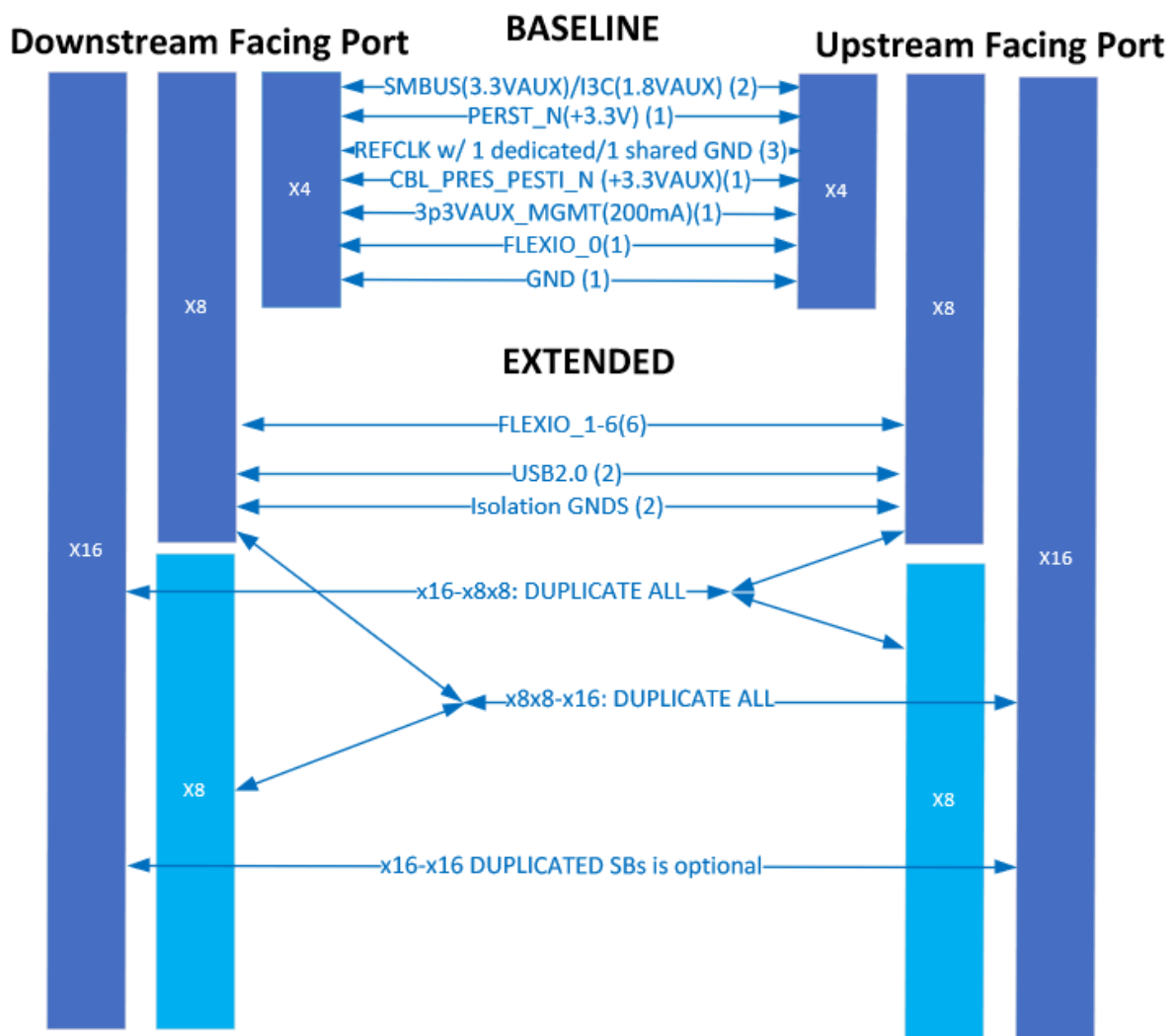
Figure 3: M-XIO sideband signal scale strategy
