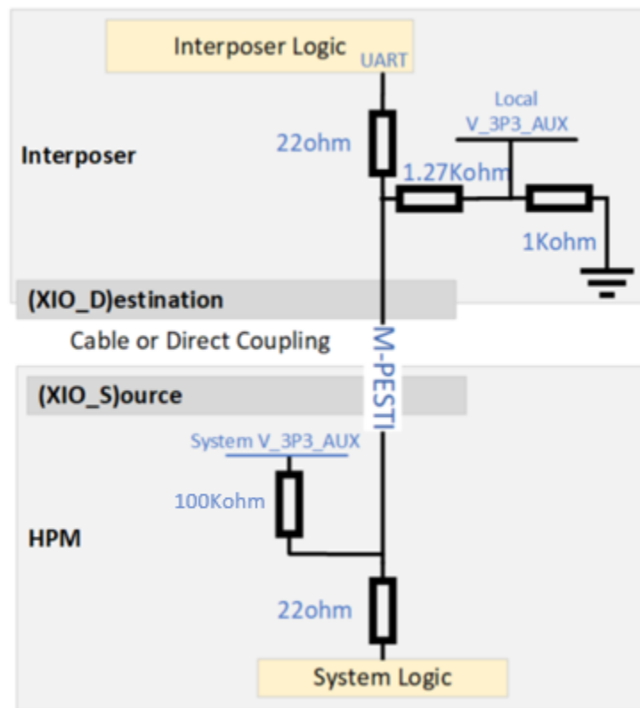
Figure 8: CBL PRES_PESTI_N Example Diagram – PESTI functionality
