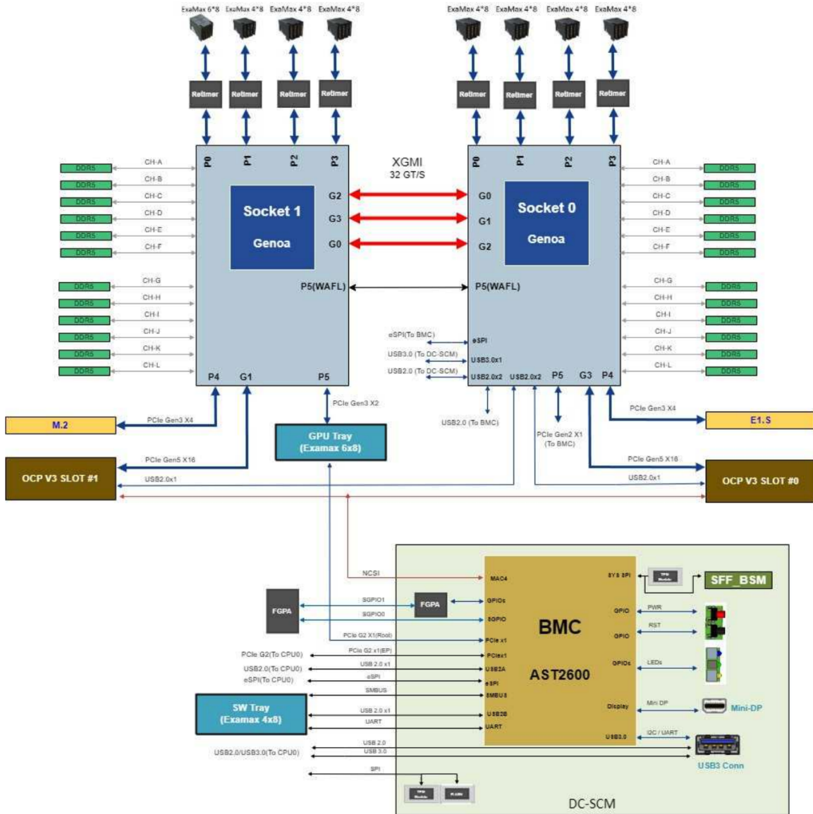
Overall block diagram of the AMD CPU Tray
