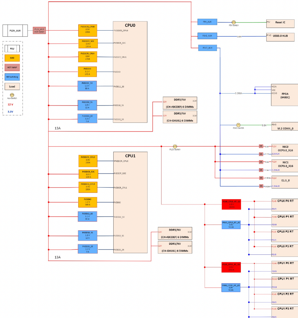
Block diagram of the CPU board power system
