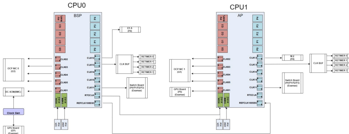
Block diagram of CPU Tray clock signals
