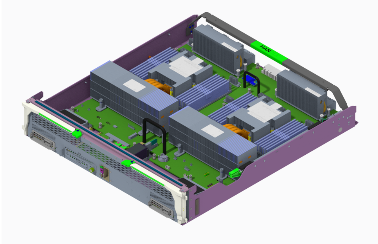
Overall view of the AMD-based CPU Tray
