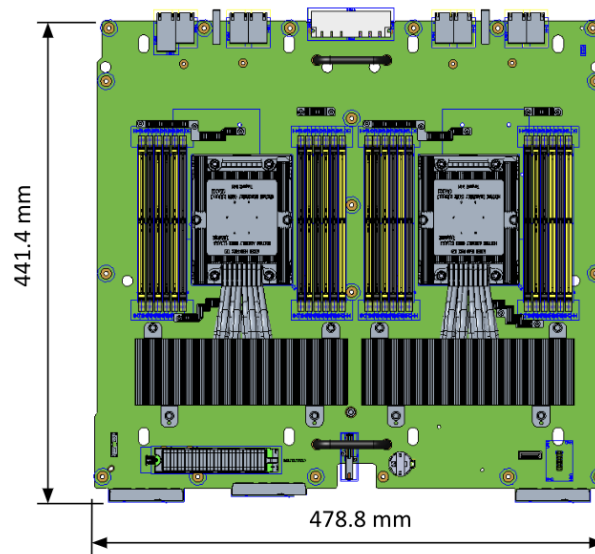
Overall dimensions of the CPU board
