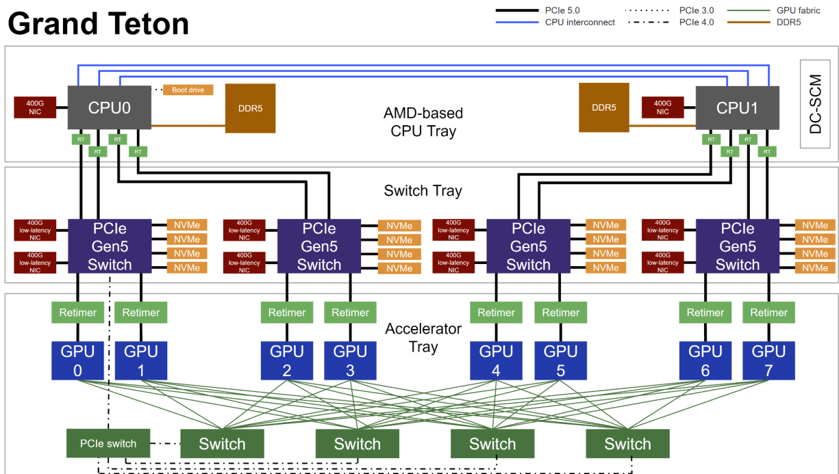
High-level block diagram of an AMD-based Grand Teton system
