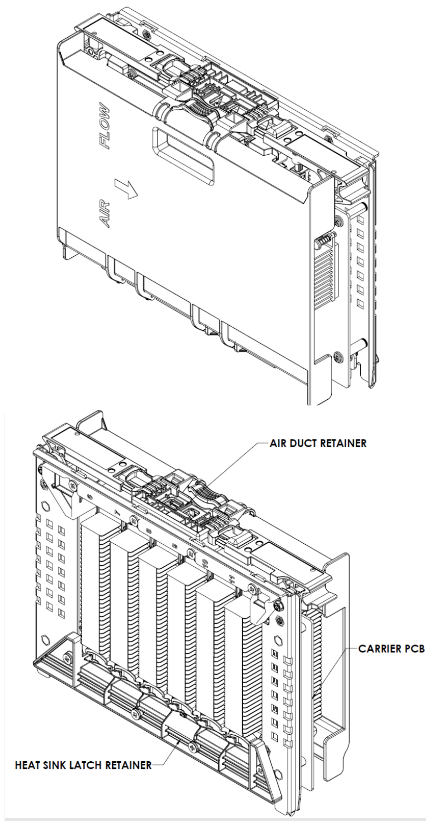
Figure 4-2 Glacier Point V2 Card Mechanical Overview
