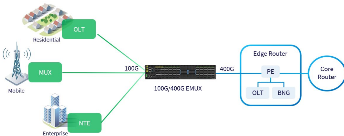
Figure 1 Large EMUX Network Topology Diagram
